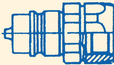
PUSH/PULL Quick Release Coupling Male with BSPP thread ISO 'B' STD
