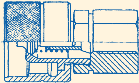
SCREW TYPE (Female) Quick Coupler BSPF (F) thread
