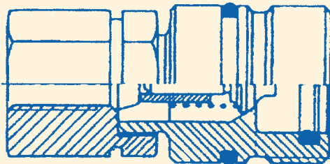
SCREW TYPE (Male) Quick Coupler BSPF (F) thread
